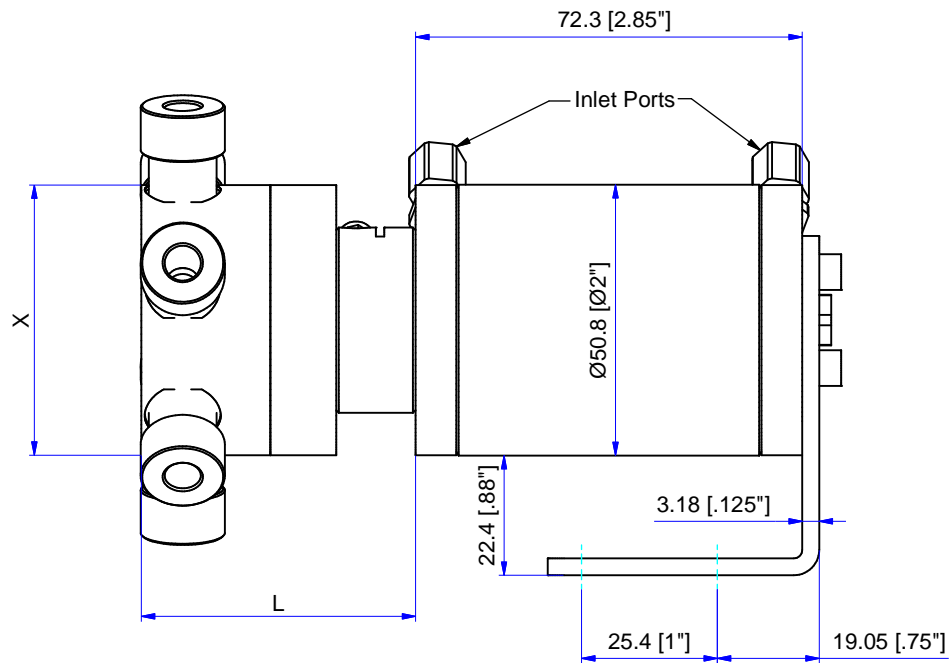
C42-9786A valve, 6 port 2-pos., shown
